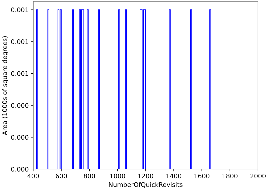
too_elab_r8_d2_griz_v3.4_10yrs : NumberOfQuickRevisits
