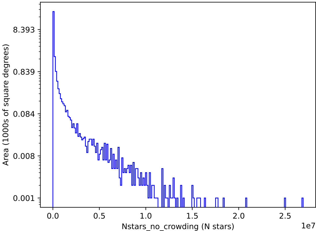
too_elab_r8_d2_griz_v3.4_10yrs i: Nstars_no_crowding
