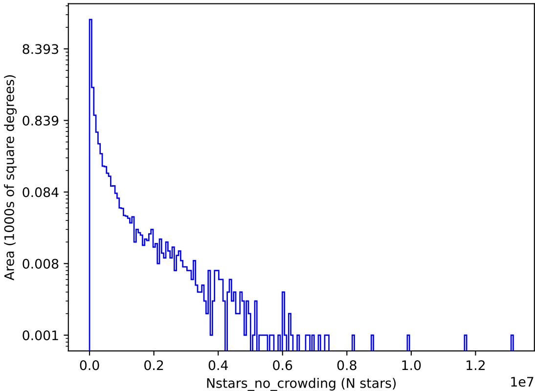
too_elab_r8_d2_griz_v3.4_10yrs g: Nstars_no_crowding
