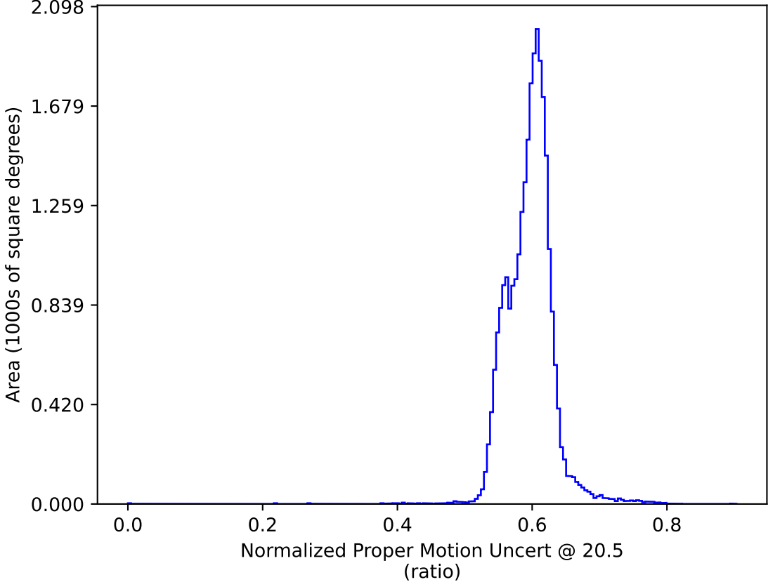
too_elab_r8_d2_griz_v3.4_10yrs : Normalized Proper Motion Uncert @ 20.5
