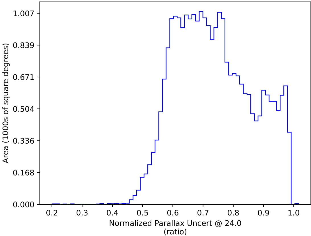
too_elab_r8_d2_griz_v3.4_10yrs : Normalized Parallax Uncert @ 24.0
