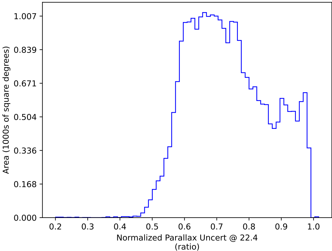
too_elab_r8_d2_griz_v3.4_10yrs : Normalized Parallax Uncert @ 22.4
