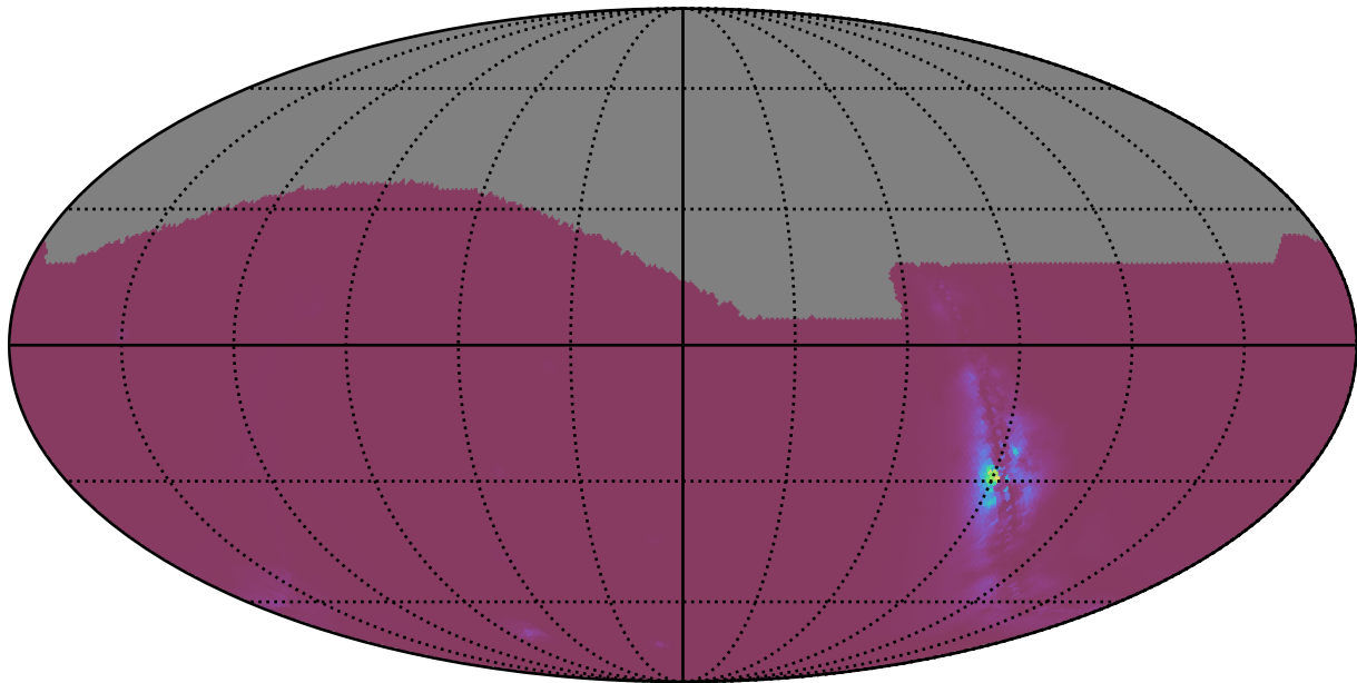
too_elab_r8_d2_griz_v3.4_10yrs : NlcPoints
