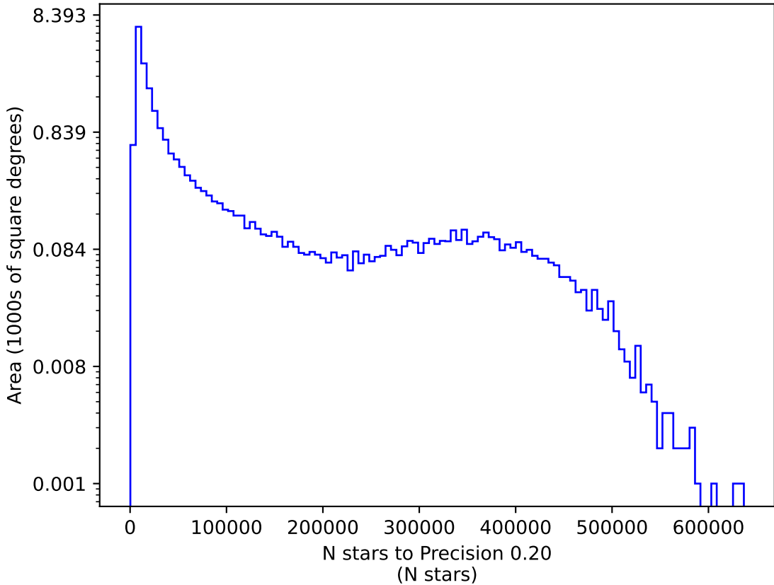
too_elab_r8_d2_griz_v3.4_10yrs y: N stars to Precision 0.20
