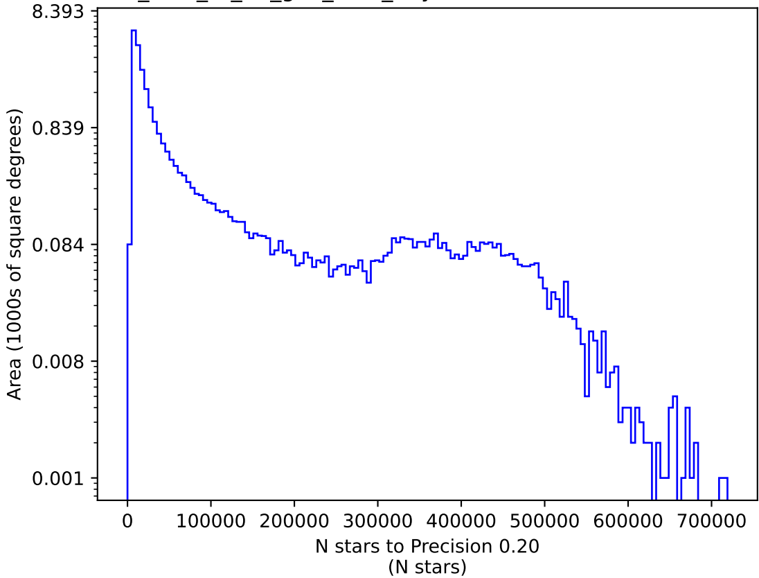
too_elab_r8_d2_griz_v3.4_10yrs i: N stars to Precision 0.20
