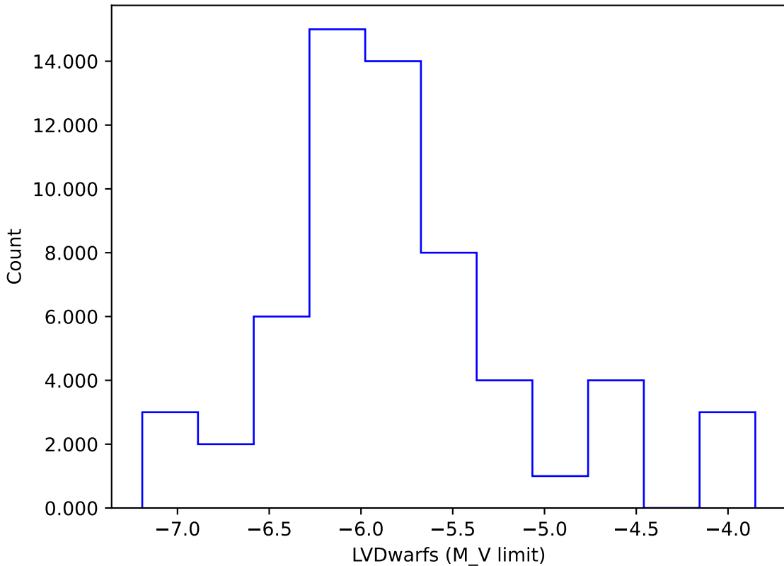
too_elab_r8_d2_griz_v3.4_10yrs gi: LVDwarfs
