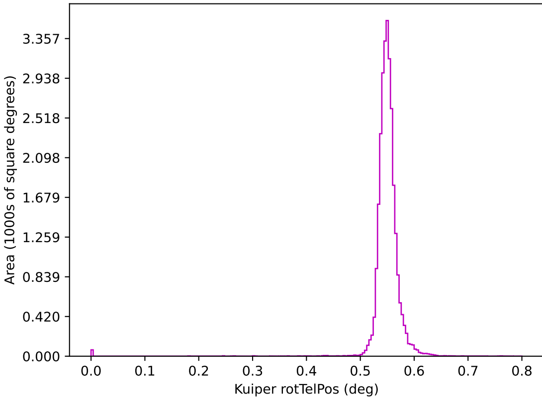
too_elab_r8_d2_griz_v3.4_10yrs z: Kuiper rotTelPos
