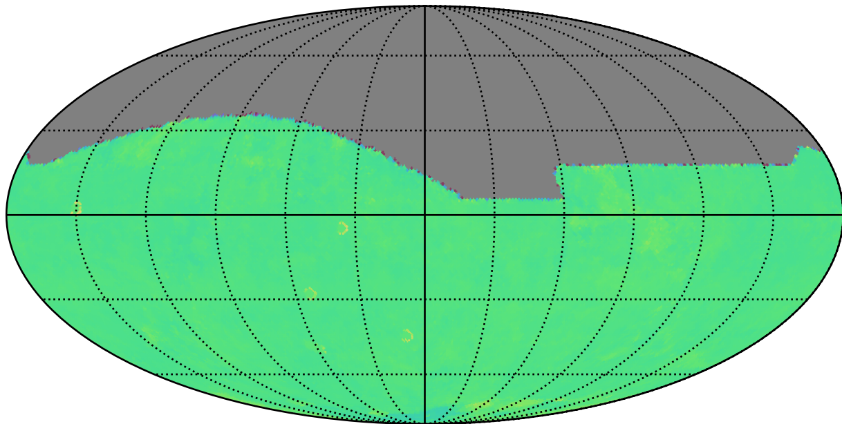
too_elab_r8_d2_griz_v3.4_10yrs r: Kuiper rotTelPos
