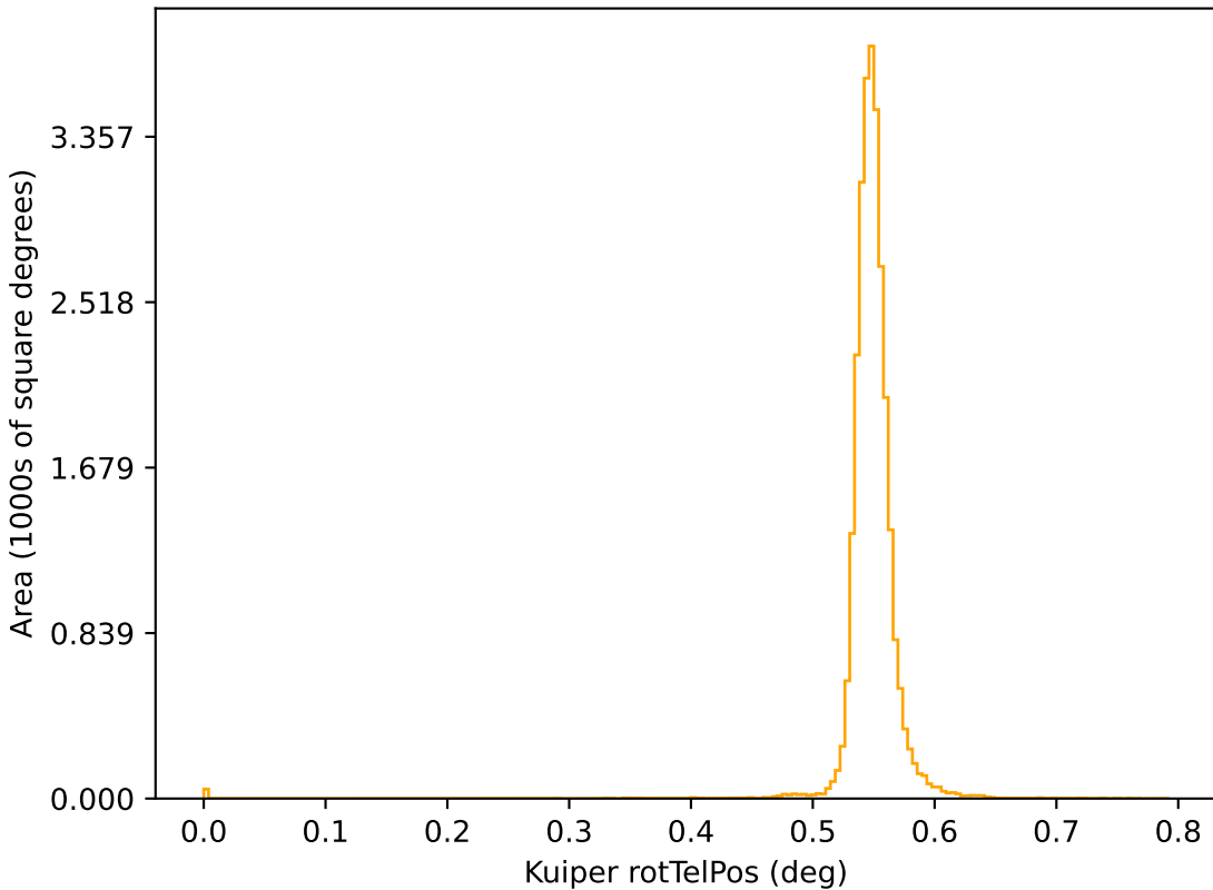
too_elab_r8_d2_griz_v3.4_10yrs r: Kuiper rotTelPos
