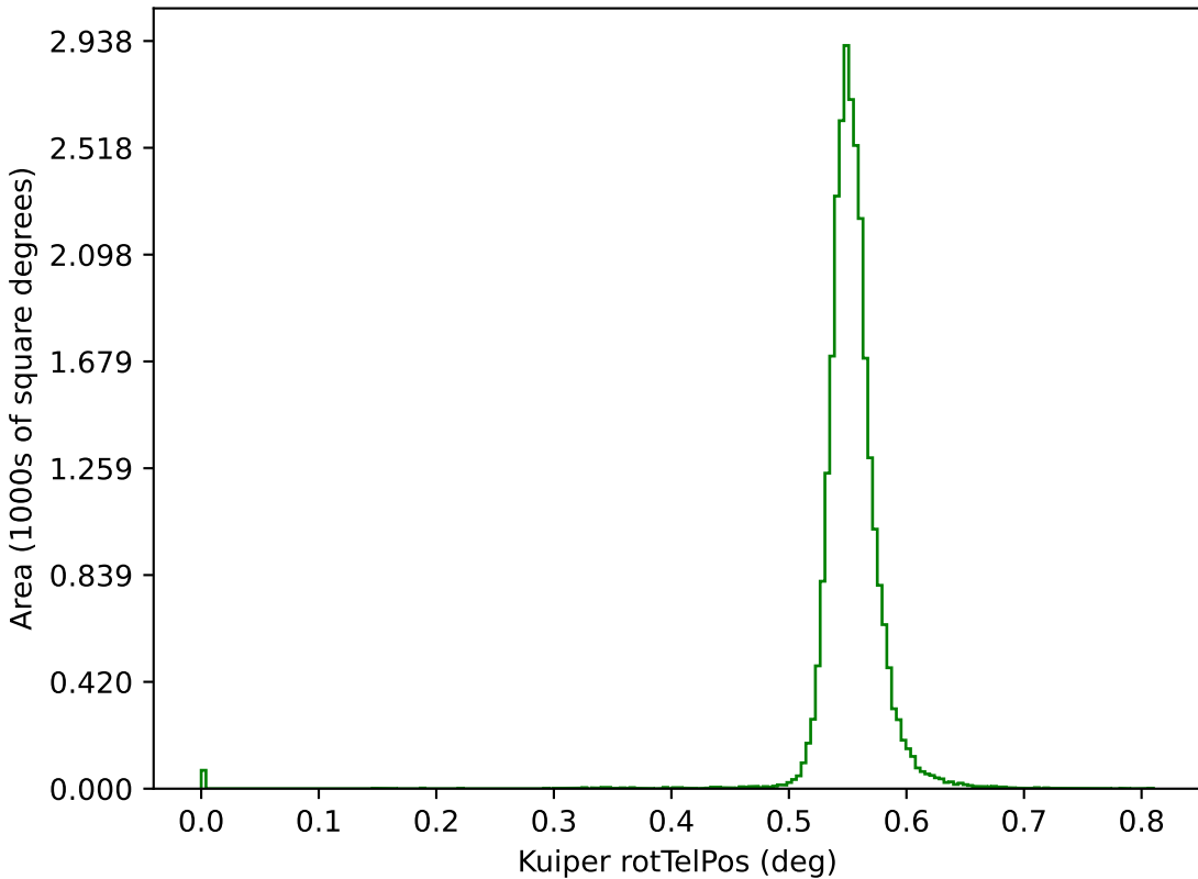
too_elab_r8_d2_griz_v3.4_10yrs g: Kuiper rotTelPos
