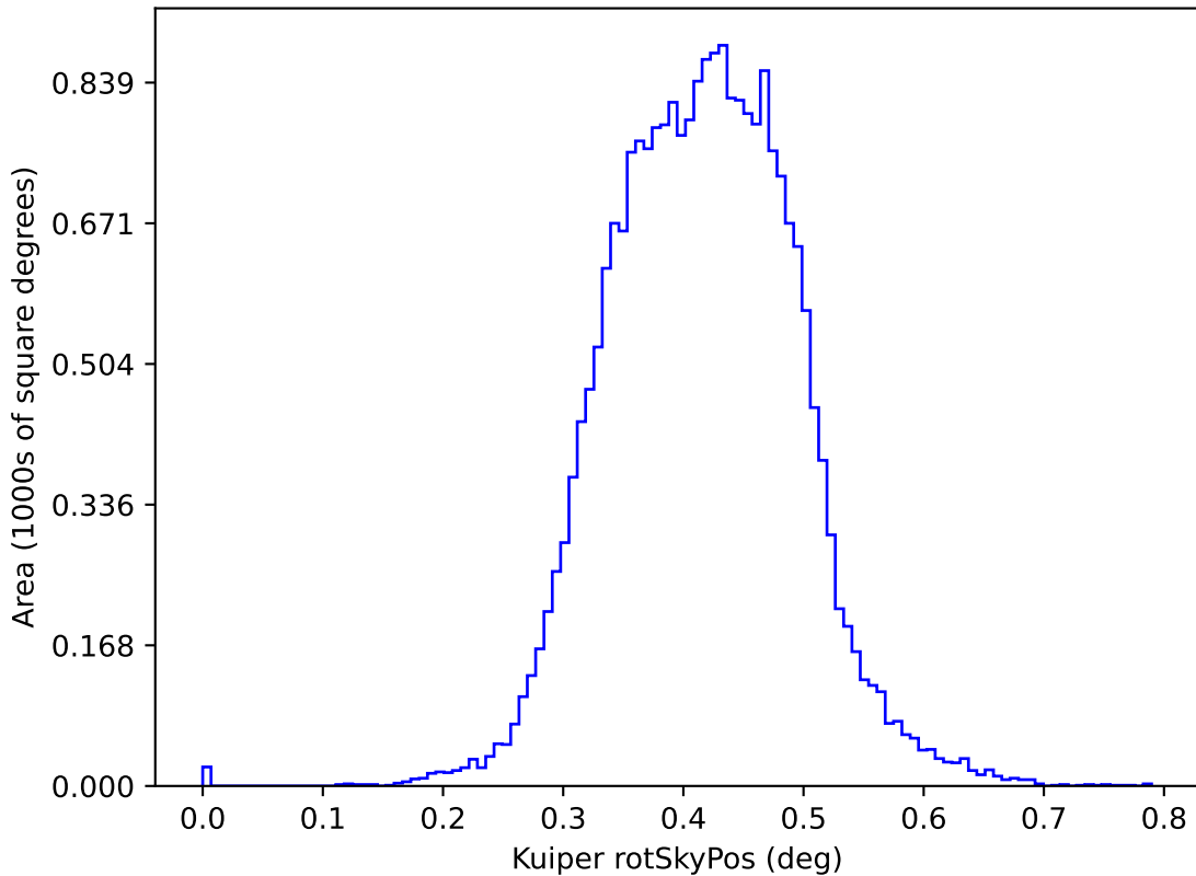
too_elab_r8_d2_griz_v3.4_10yrs y: Kuiper rotSkyPos
