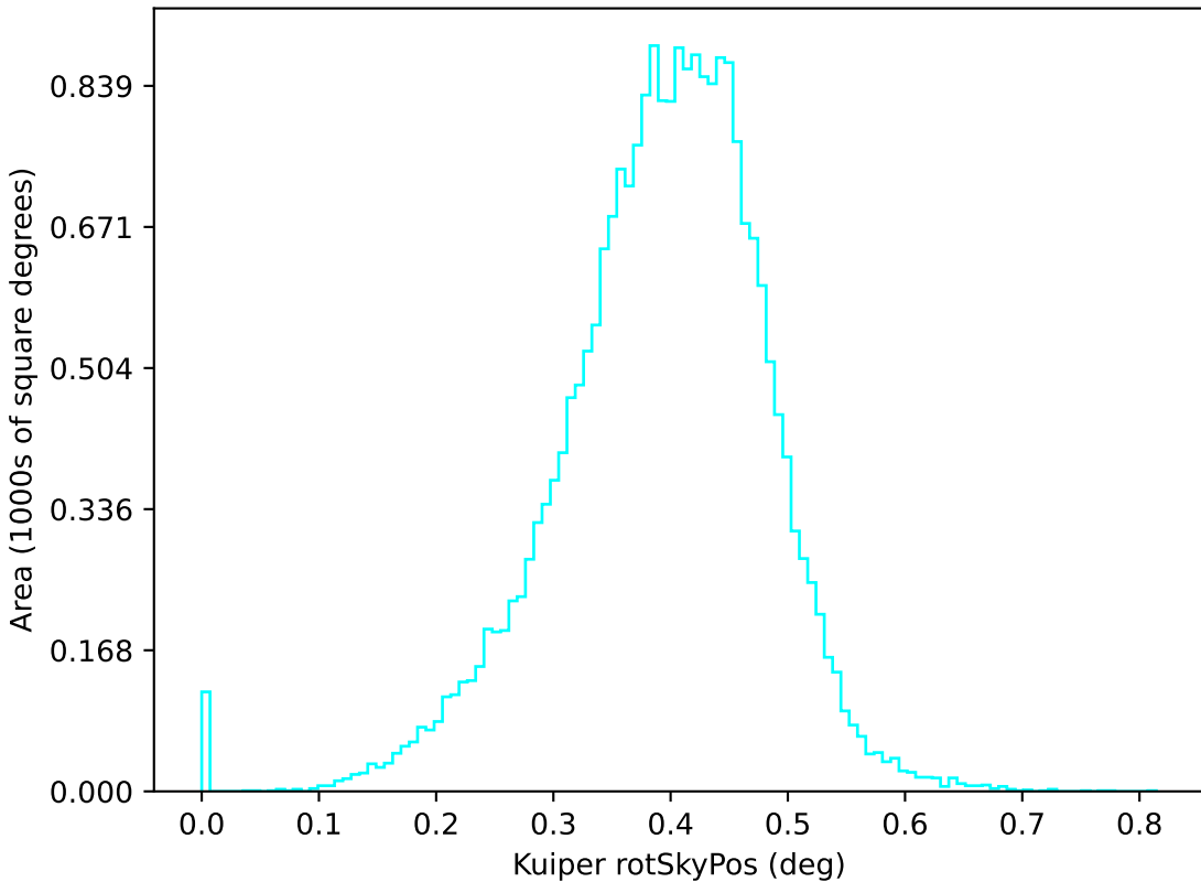
too_elab_r8_d2_griz_v3.4_10yrs u: Kuiper rotSkyPos
