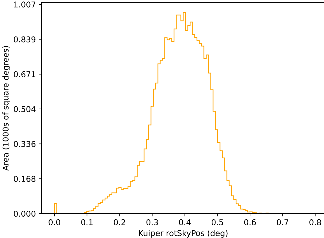
too_elab_r8_d2_griz_v3.4_10yrs r: Kuiper rotSkyPos
