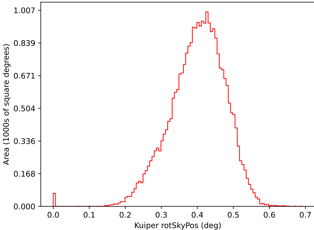
too_elab_r8_d2_griz_v3.4_10yrs i: Kuiper rotSkyPos
