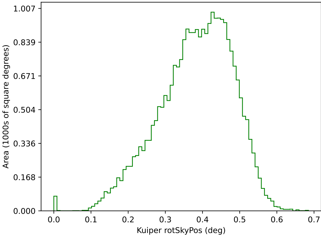
too_elab_r8_d2_griz_v3.4_10yrs g: Kuiper rotSkyPos
