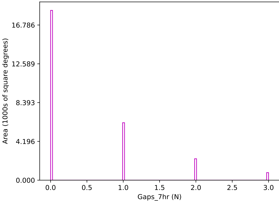
too_elab_r8_d2_griz_v3.4_10yrs z band: Gaps_7hr
