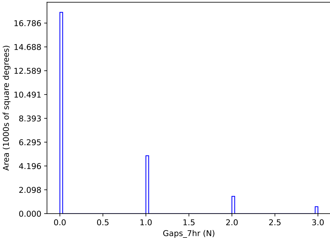
too_elab_r8_d2_griz_v3.4_10yrs y band: Gaps_7hr
