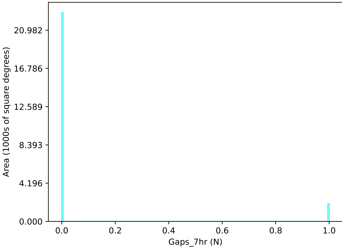
too_elab_r8_d2_griz_v3.4_10yrs u band: Gaps_7hr
