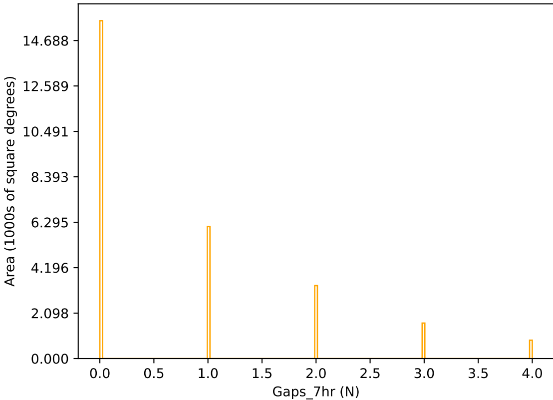
too_elab_r8_d2_griz_v3.4_10yrs r band: Gaps_7hr
