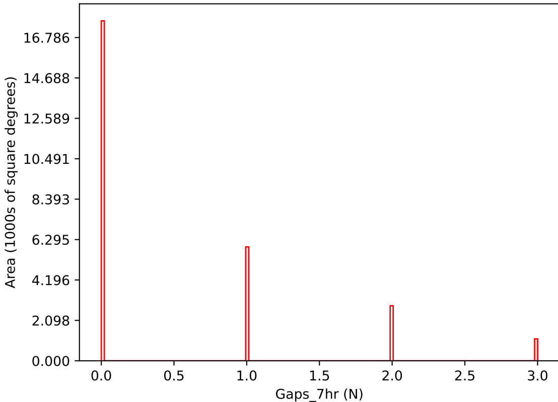
too_elab_r8_d2_griz_v3.4_10yrs i band: Gaps_7hr
