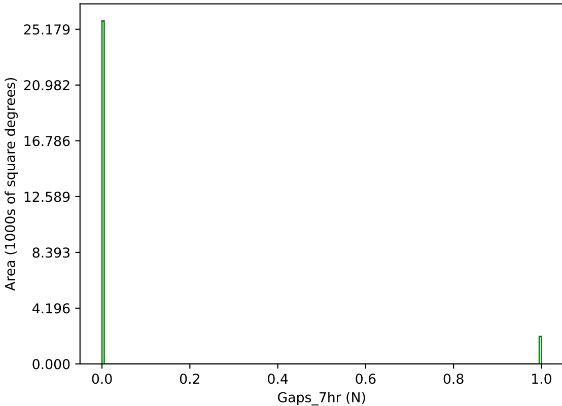
too_elab_r8_d2_griz_v3.4_10yrs g band: Gaps_7hr
