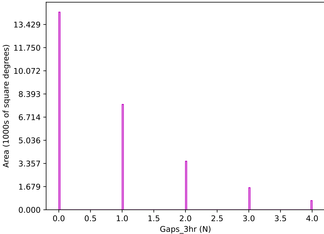
too_elab_r8_d2_griz_v3.4_10yrs z band: Gaps_3hr
