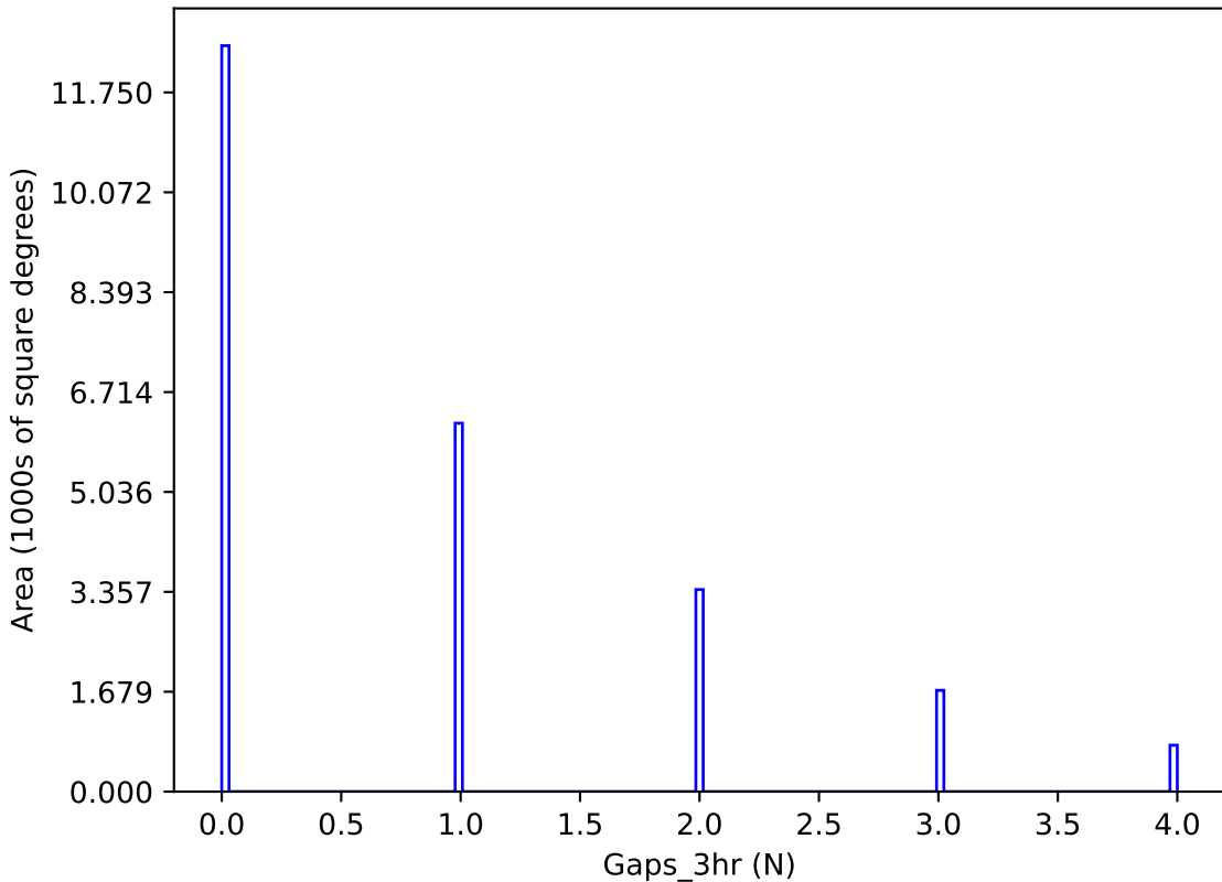
too_elab_r8_d2_griz_v3.4_10yrs y band: Gaps_3hr
