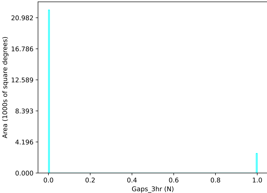
too_elab_r8_d2_griz_v3.4_10yrs u band: Gaps_3hr
