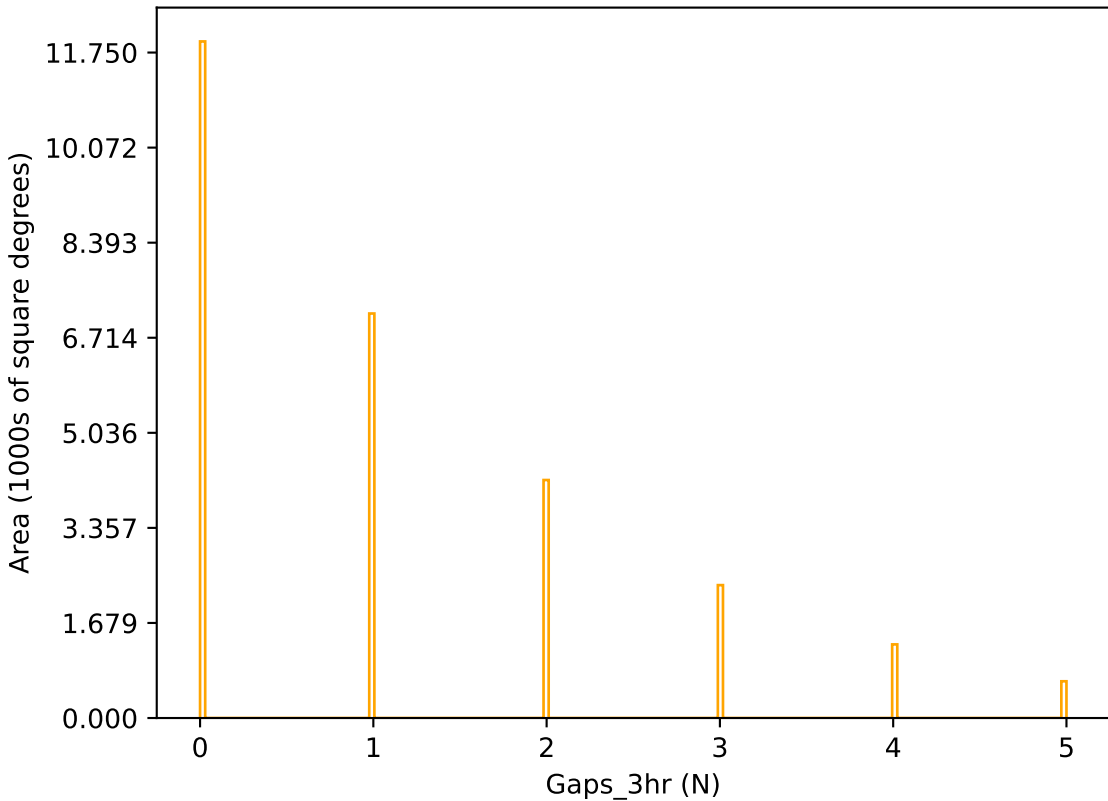
too_elab_r8_d2_griz_v3.4_10yrs r band: Gaps_3hr
