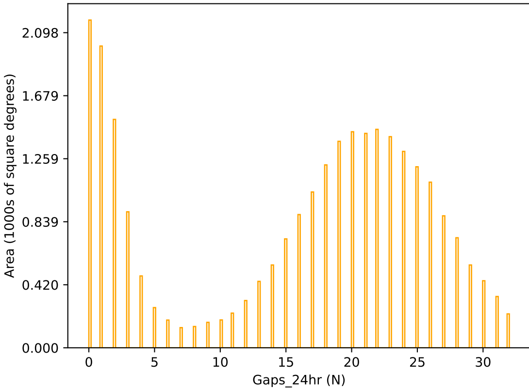
too_elab_r8_d2_griz_v3.4_10yrs r band: Gaps_24hr
