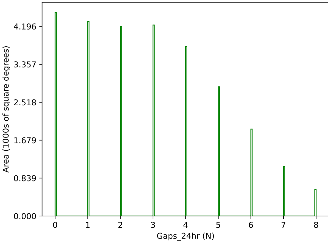
too_elab_r8_d2_griz_v3.4_10yrs g band: Gaps_24hr
