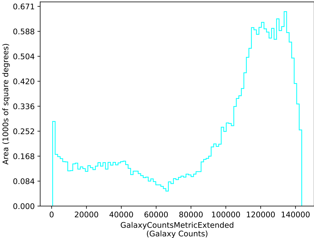
too_elab_r8_d2_griz_v3.4_10yrs u: GalaxyCountsMetricExtended
