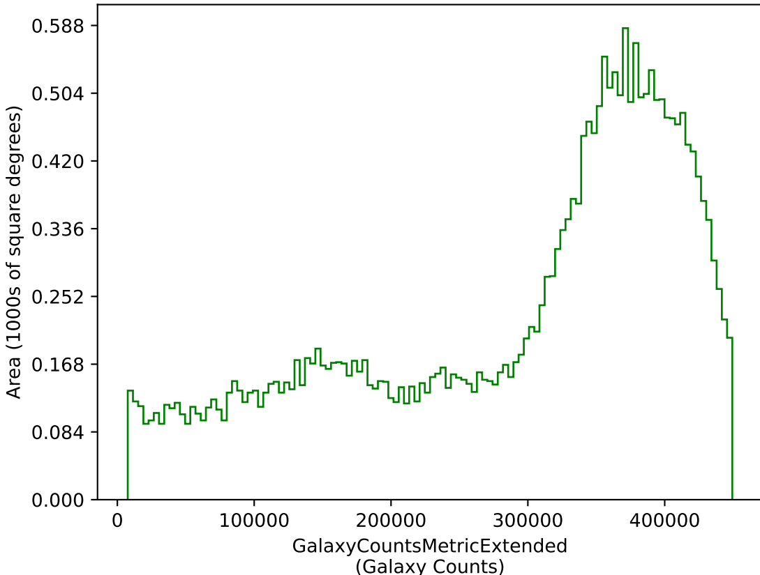
too_elab_r8_d2_griz_v3.4_10yrs g: GalaxyCountsMetricExtended
