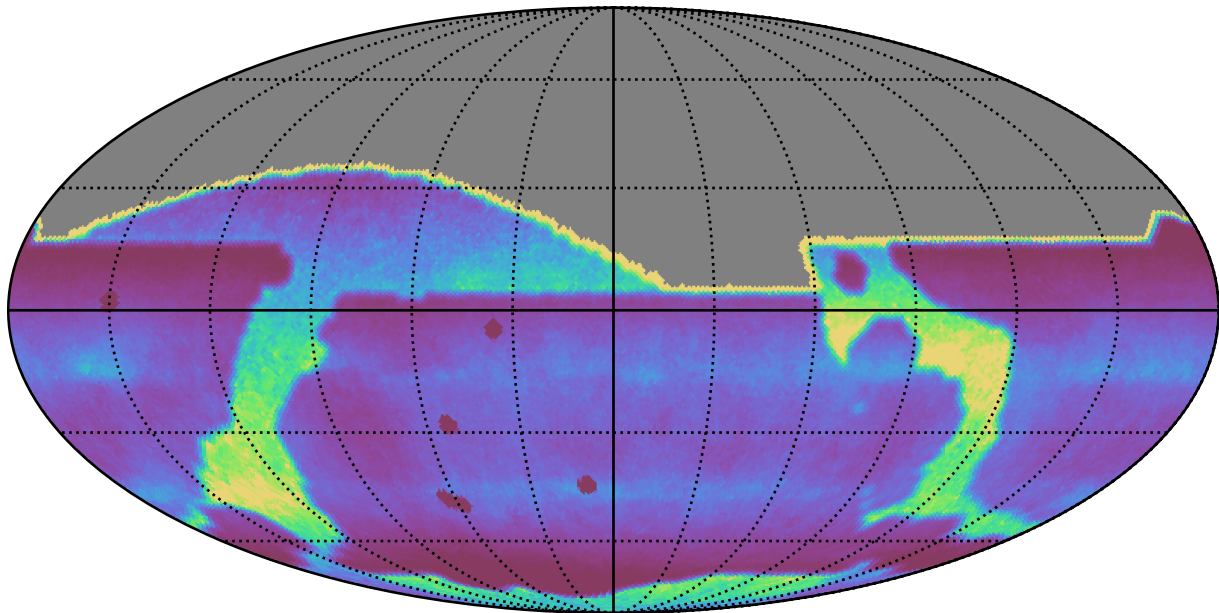
too_elab_r8_d2_griz_v3.4_10yrs : DCRprecision
