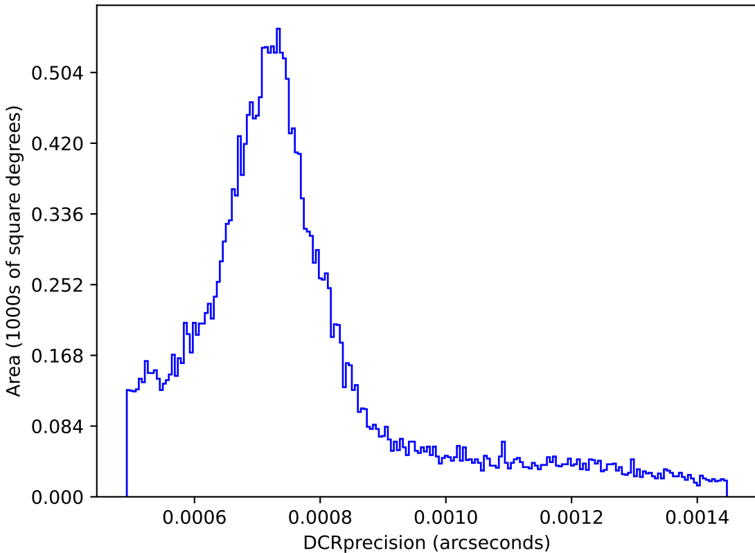
too_elab_r8_d2_griz_v3.4_10yrs : DCRprecision
