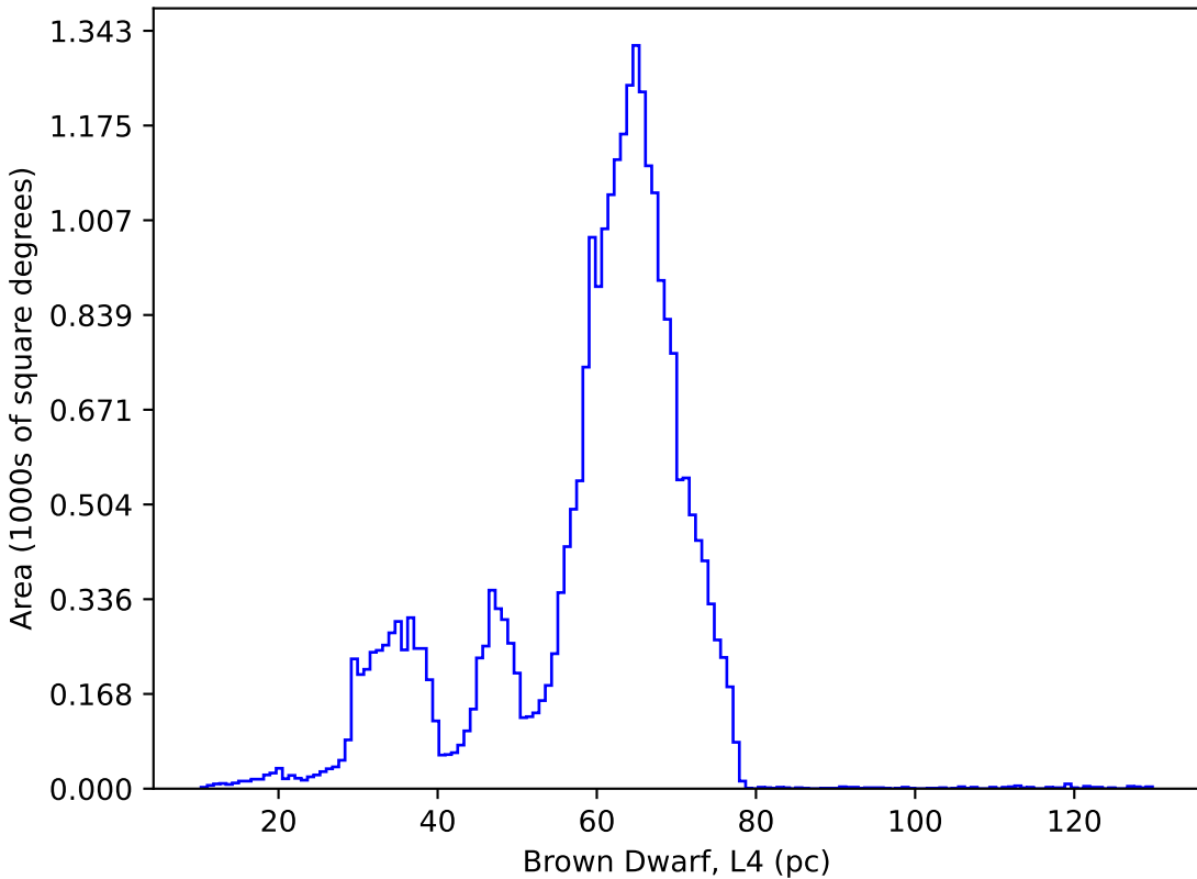
too_elab_r8_d2_griz_v3.4_10yrs : Brown Dwarf, L4
