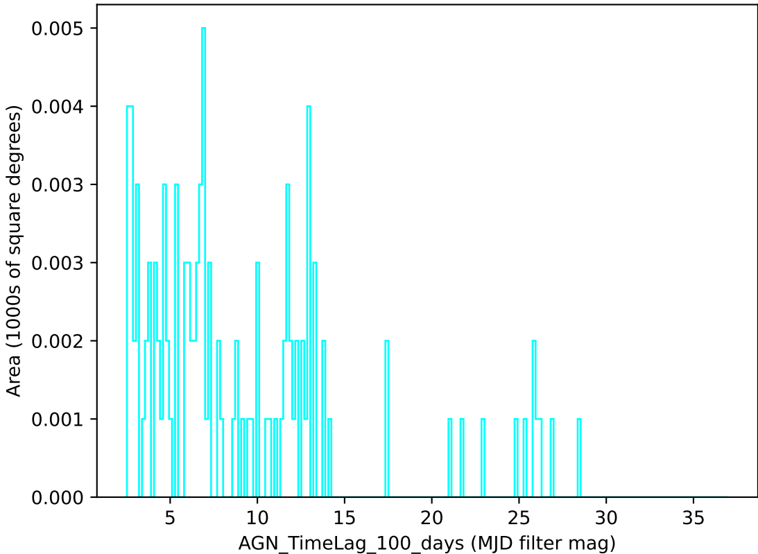
too_elab_r8_d2_griz_v3.4_10yrs u band: AGN_TimeLag_100_days
