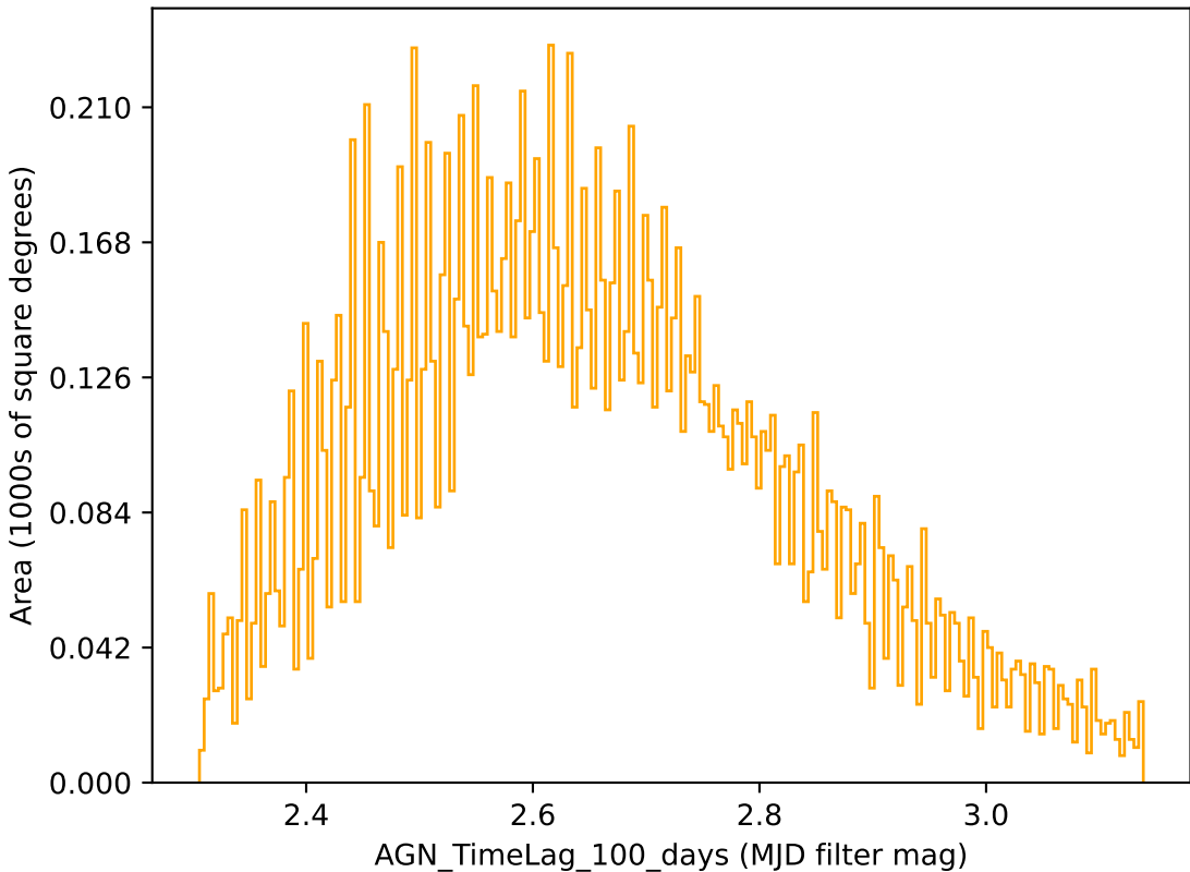
too_elab_r8_d2_griz_v3.4_10yrs r band: AGN_TimeLag_100_days
