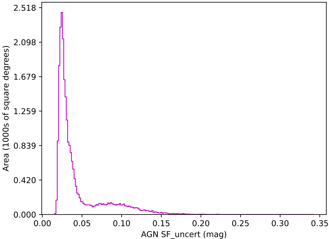
too_elab_r8_d2_griz_v3.4_10yrs z band: AGN SF_uncert
