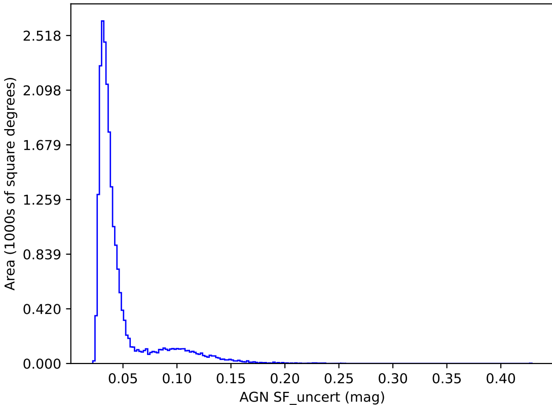
too_elab_r8_d2_griz_v3.4_10yrs y band: AGN SF_uncert
