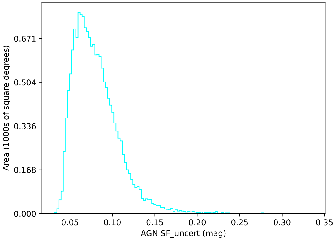
too_elab_r8_d2_griz_v3.4_10yrs u band: AGN SF_uncert
