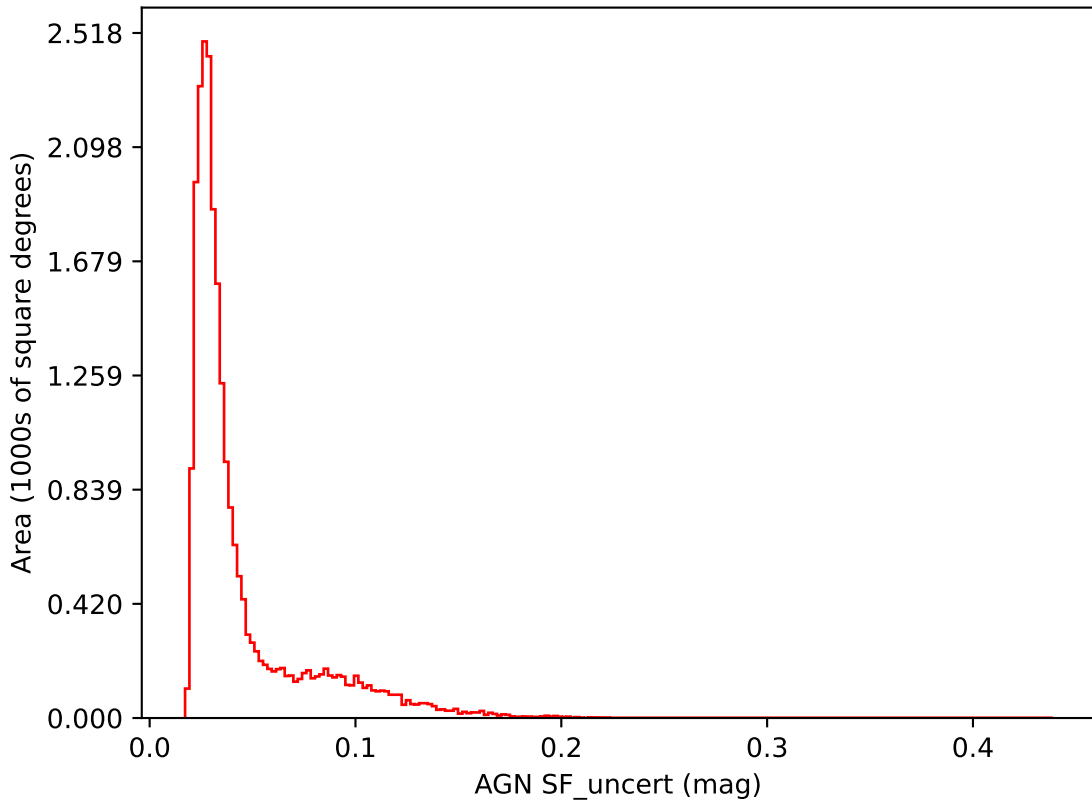
too_elab_r8_d2_griz_v3.4_10yrs i band: AGN SF_uncert
