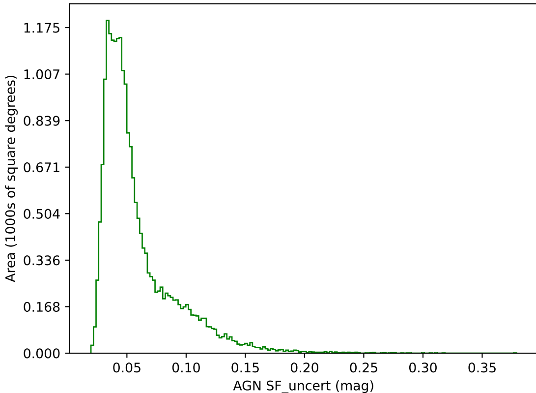
too_elab_r8_d2_griz_v3.4_10yrs g band: AGN SF_uncert
