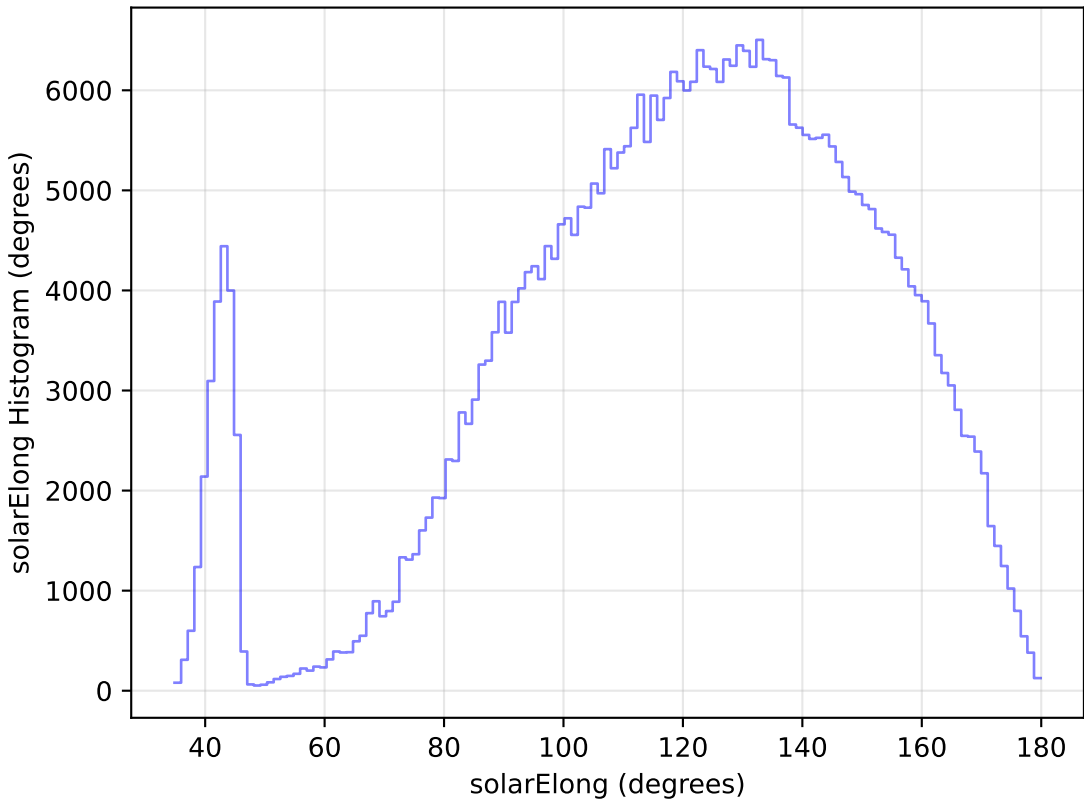
too_elab_r8_d2_griz_v3.4_10yrs WFD z band: solarElong Histogram
