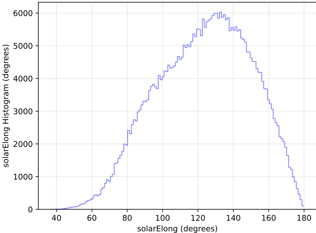
too_elab_r8_d2_griz_v3.4_10yrs WFD y band: solarElong Histogram
