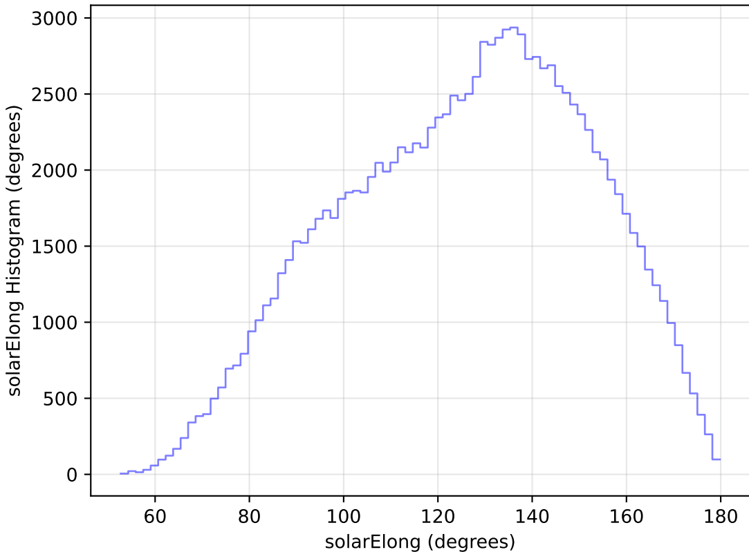
too_elab_r8_d2_griz_v3.4_10yrs WFD u band: solarElong Histogram
