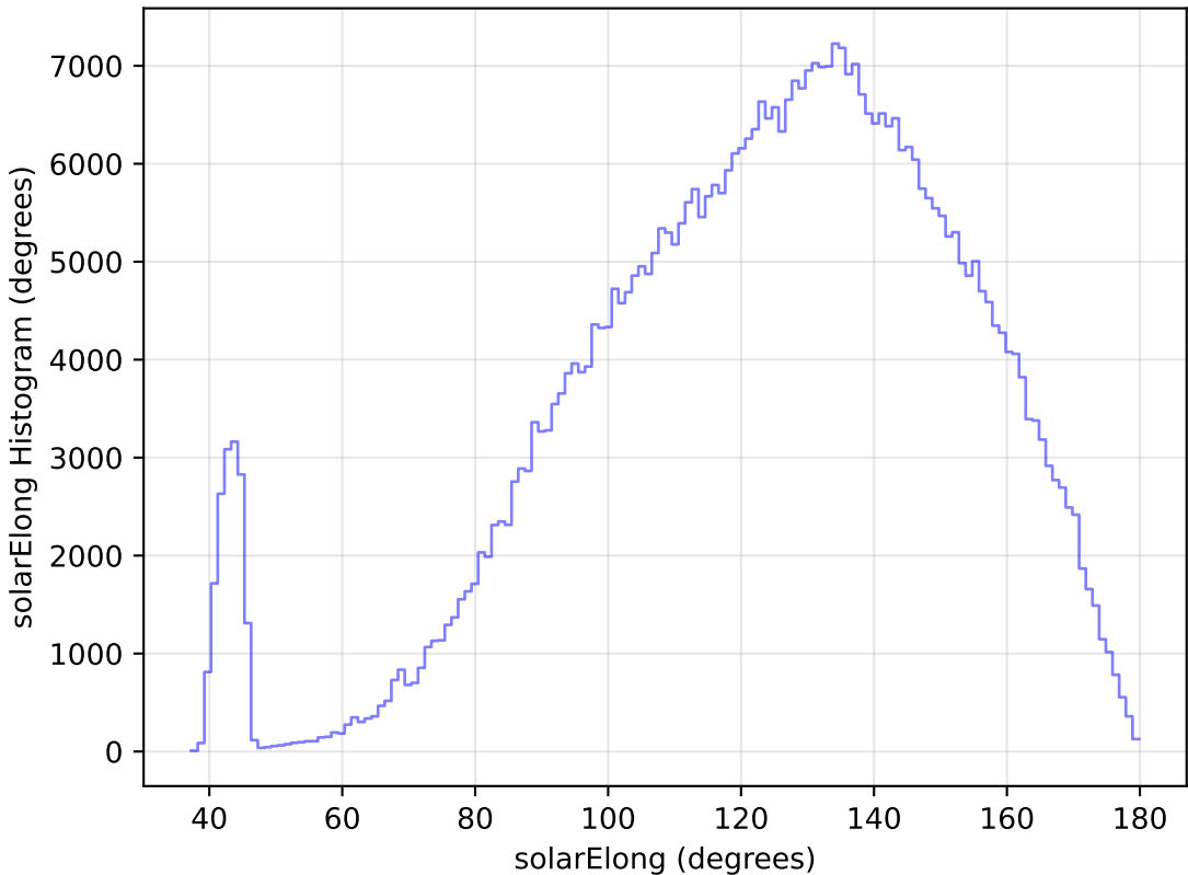
too_elab_r8_d2_griz_v3.4_10yrs WFD r band: solarElong Histogram
