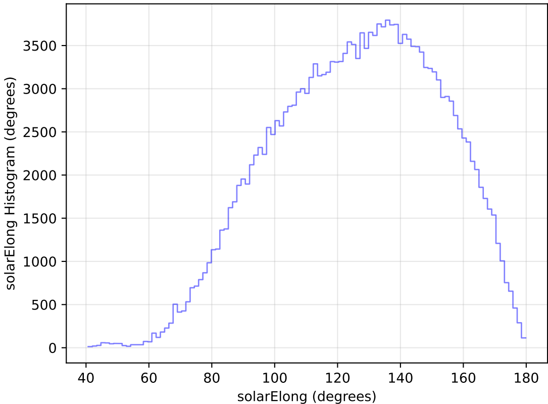
too_elab_r8_d2_griz_v3.4_10yrs WFD g band: solarElong Histogram
