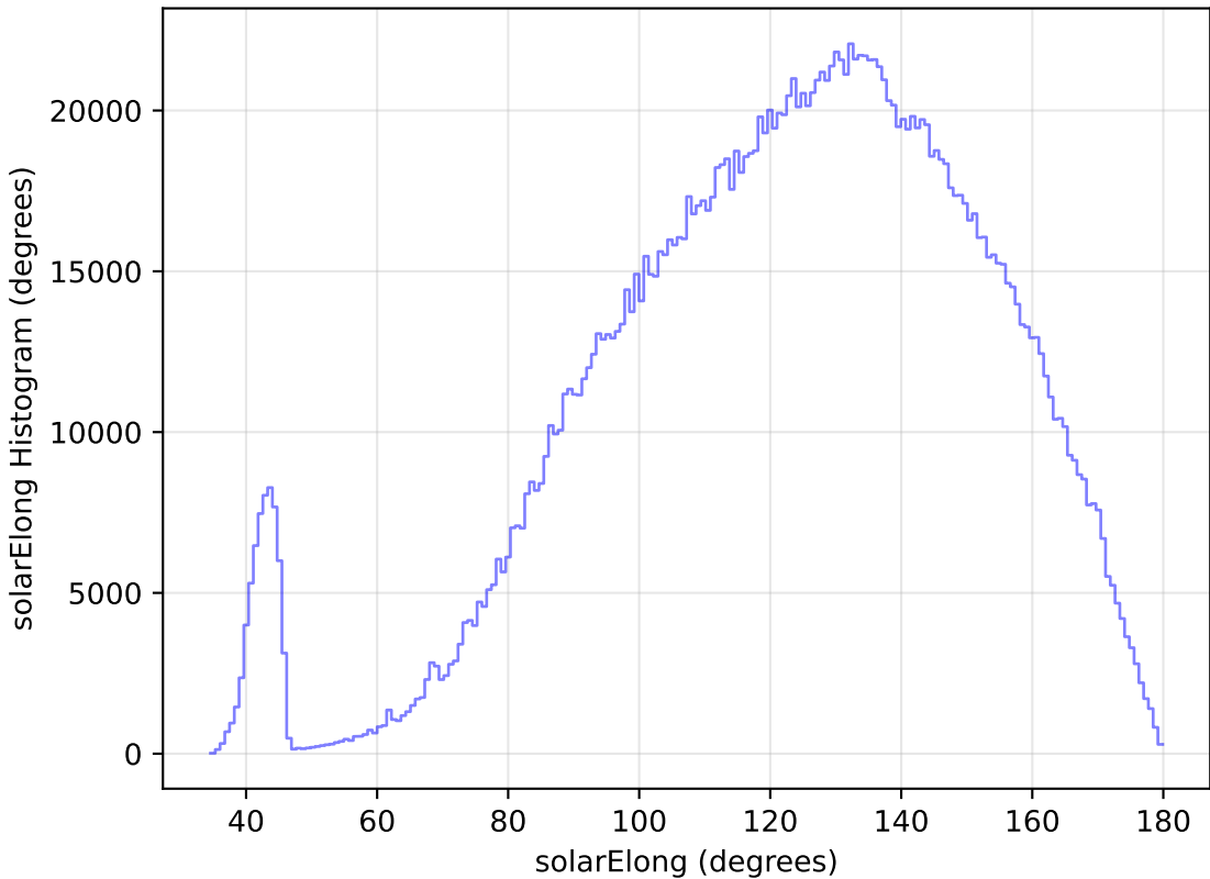
too_elab_r8_d2_griz_v3.4_10yrs WFD all bands: solarElong Histogram
