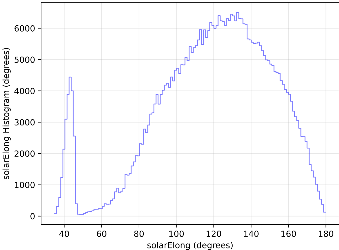
too_elab_r8_d2_griz_v3.4_10yrs All sky z band: solarElong Histogram
